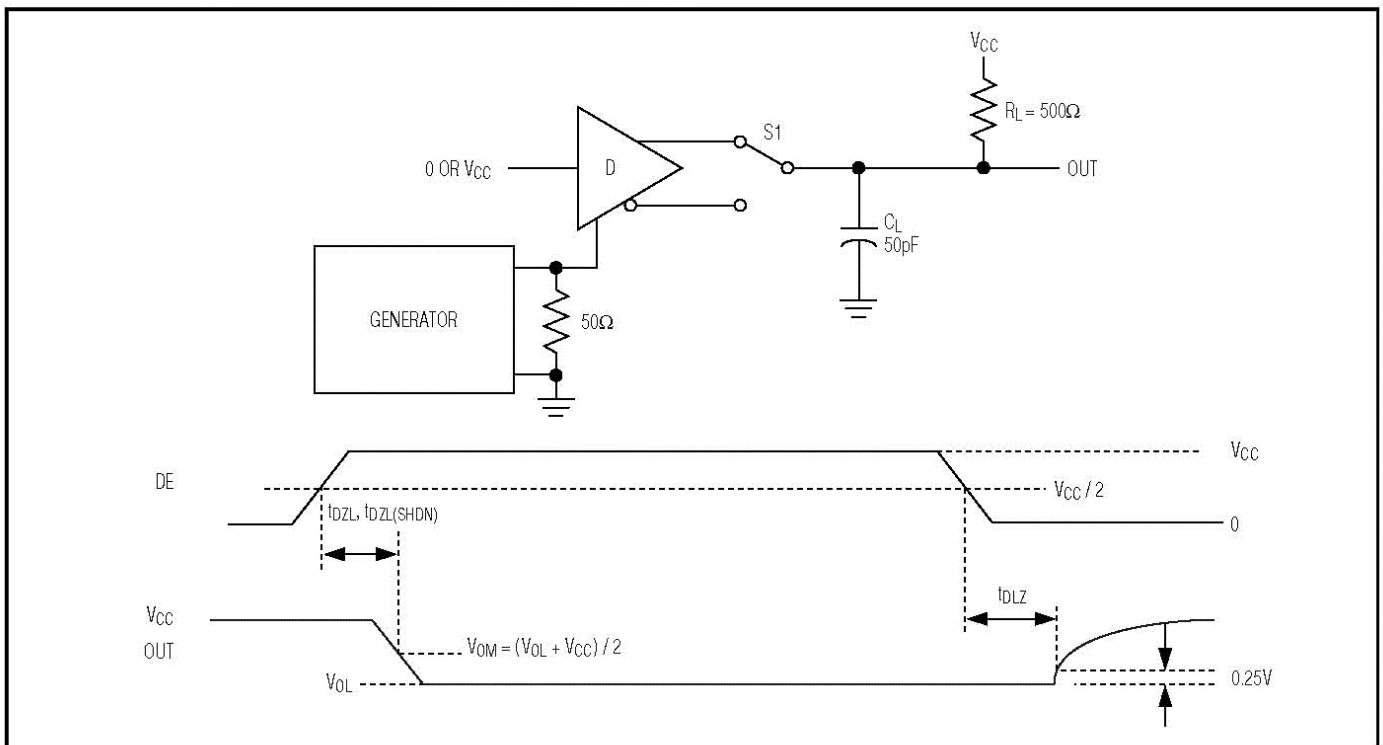
Figure 5. Driver Enable and Disable Times ( t_{DZL} , t_{DZL(SHDN)} , t_{DLZ} )
